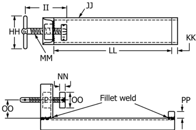
FIG. 3 Device for Detaching 1-in. [25-mm] Square by 11¼-in. [285-mm] Bars from Center Side Plate of Double Molds
