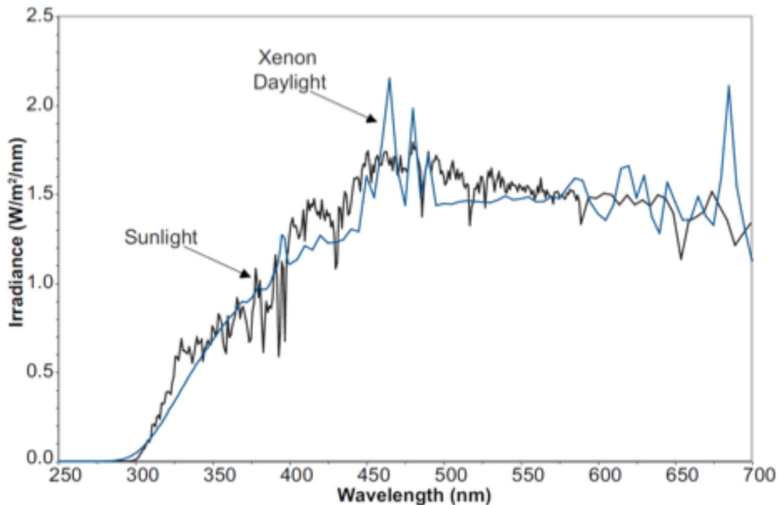
Figure #9 – Sunlight (outdoor) vs Xenon arc unit with daylight filter
